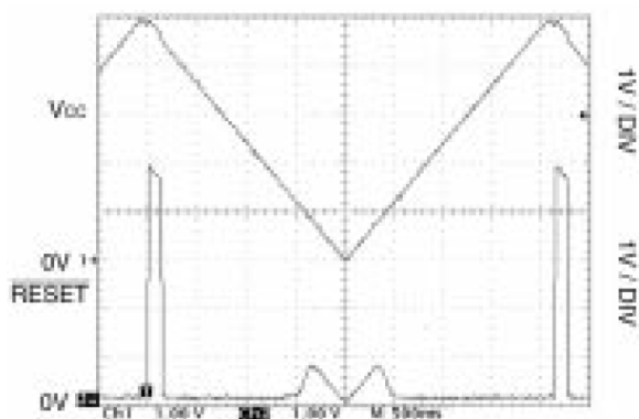
Fig. 8: SP705/707 \overline{RESET} Output Voltage vs. Supply Voltage
