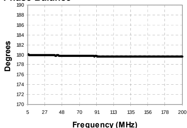
Phase Balance
