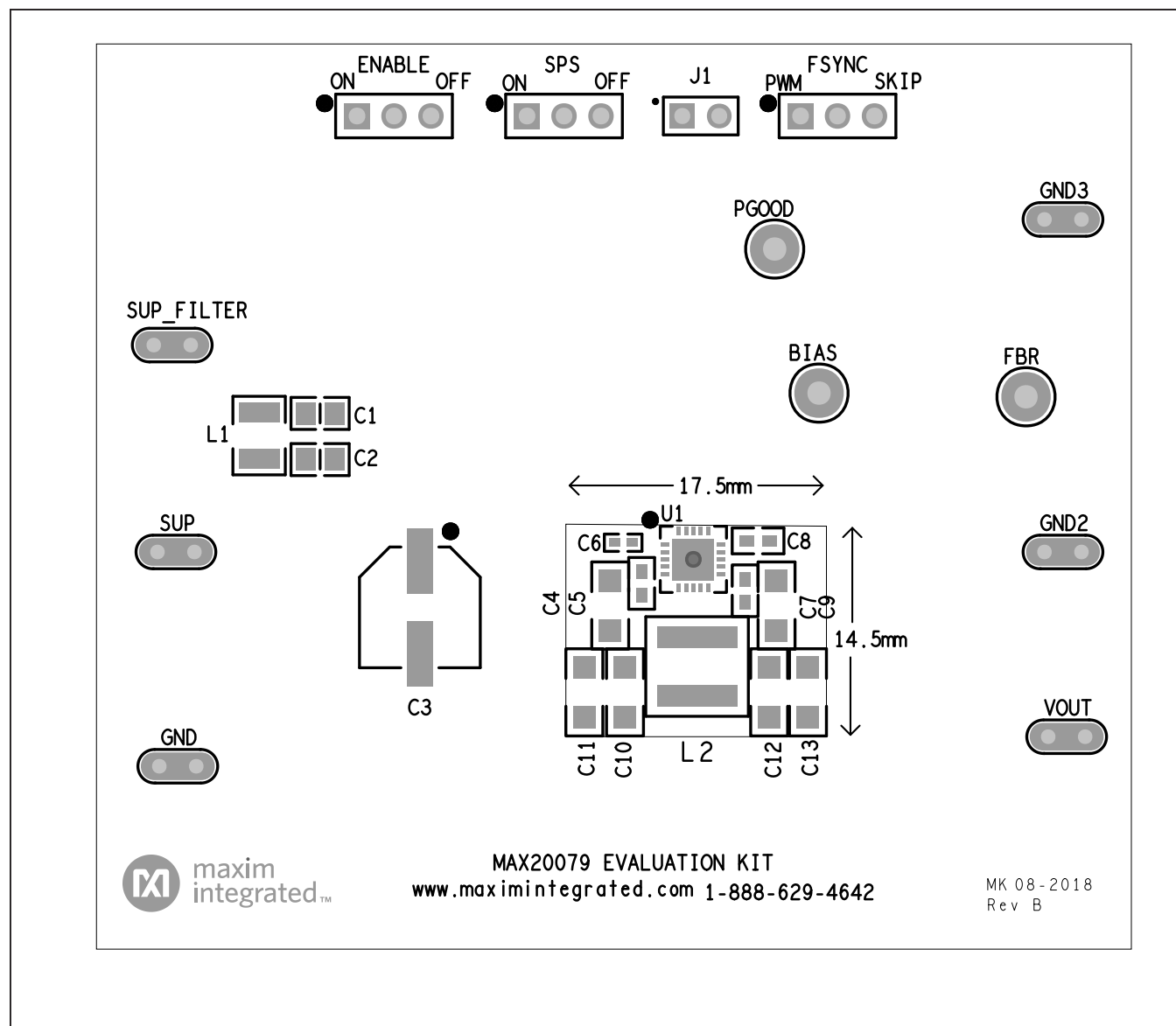
MAX20079 EVKIT Component Placement Guide Top Silk
