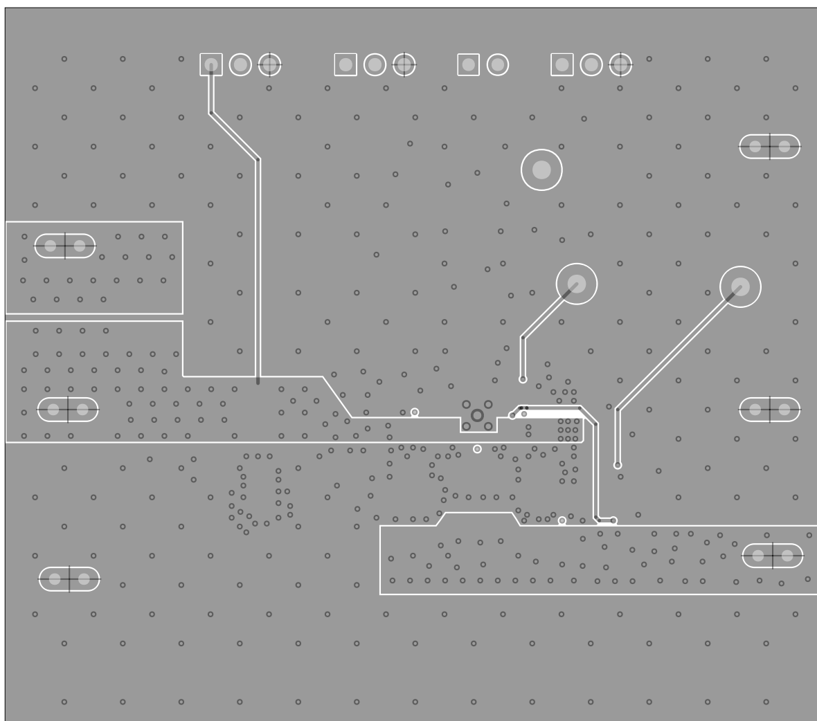
MAX20079 EVKIT PCB Layout Internal 3
