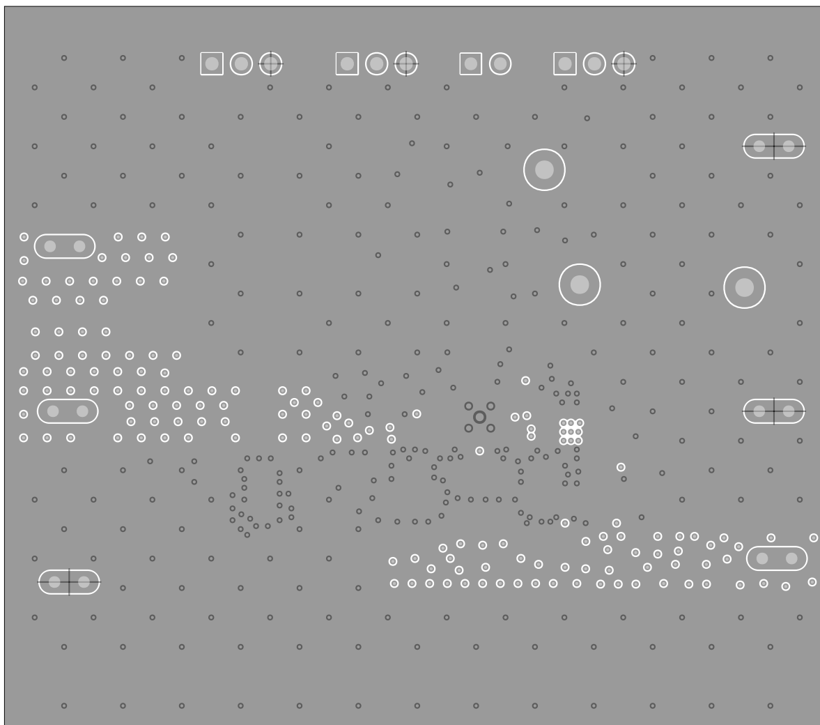
MAX20079 EVKIT Layout Internal 2
