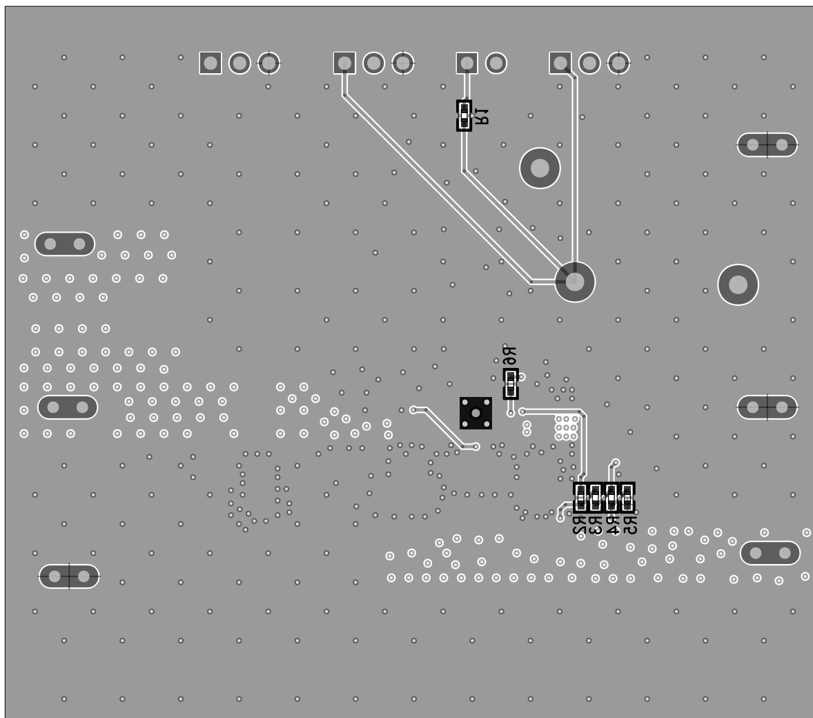
MAX20079 EVKIT Component Placement Guide Bottom
