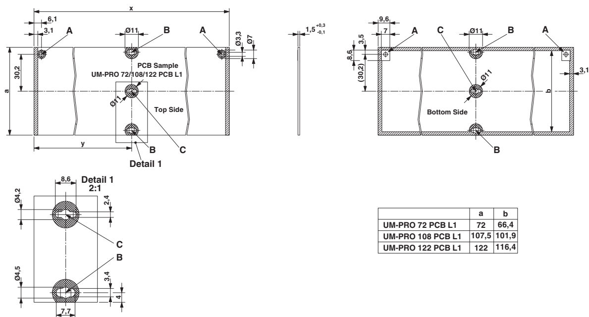
Dimensional drawing
