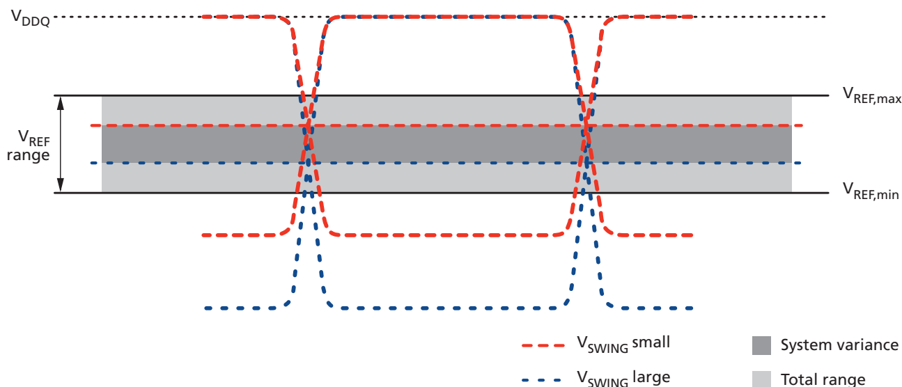
Figure 65: V REFDO Voltage Range
