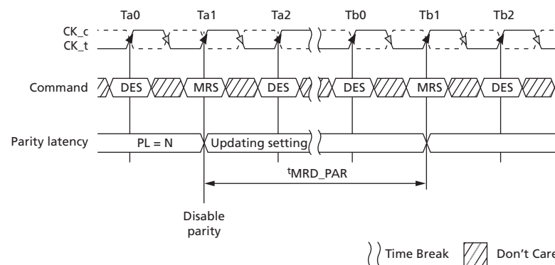
Figure 59: Parity Exit Timing Example – t_{MRD\_PAR}
