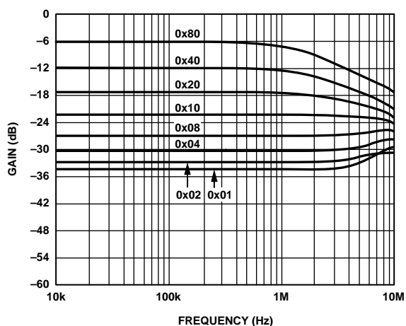
Figure 19. Gain vs. Frequency vs. Code, R_{AB} = 2.5\text{k}\Omega
