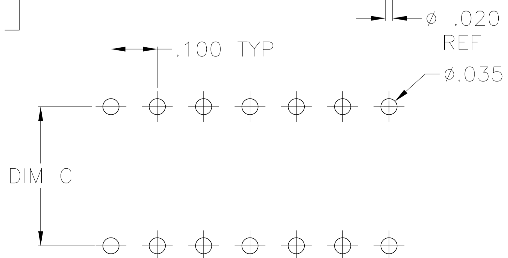
P.C.B. HOLE LAYOUT TOLERANCE \pm .003
