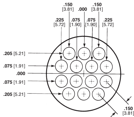
Arrangement 22-14 Max. Wire Ins. Dia. = .100 [2.54]
