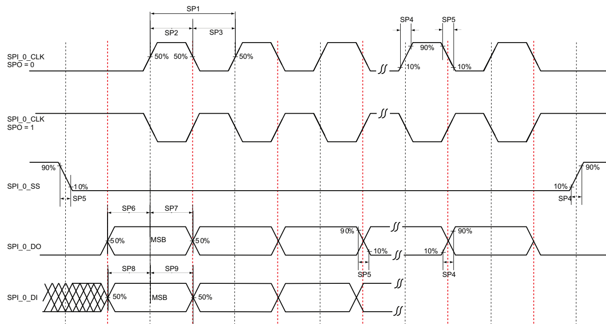
Figure 18 • SPI Timing for a Single Frame Transfer in Motorola Mode (SPH = 1)
