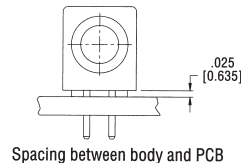
Spacing between body and PCB
