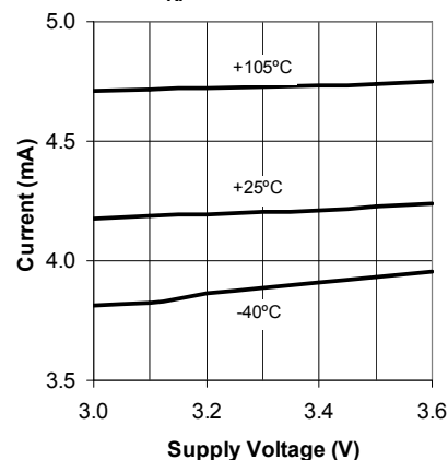
Current vs. Supply Voltage f_{RF} = 315MHz
