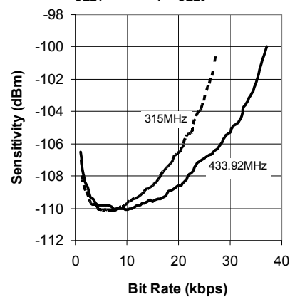
Sensitivity at 1% BER V_{SEL1} = 3.3V, V_{SEL0} = 0V
