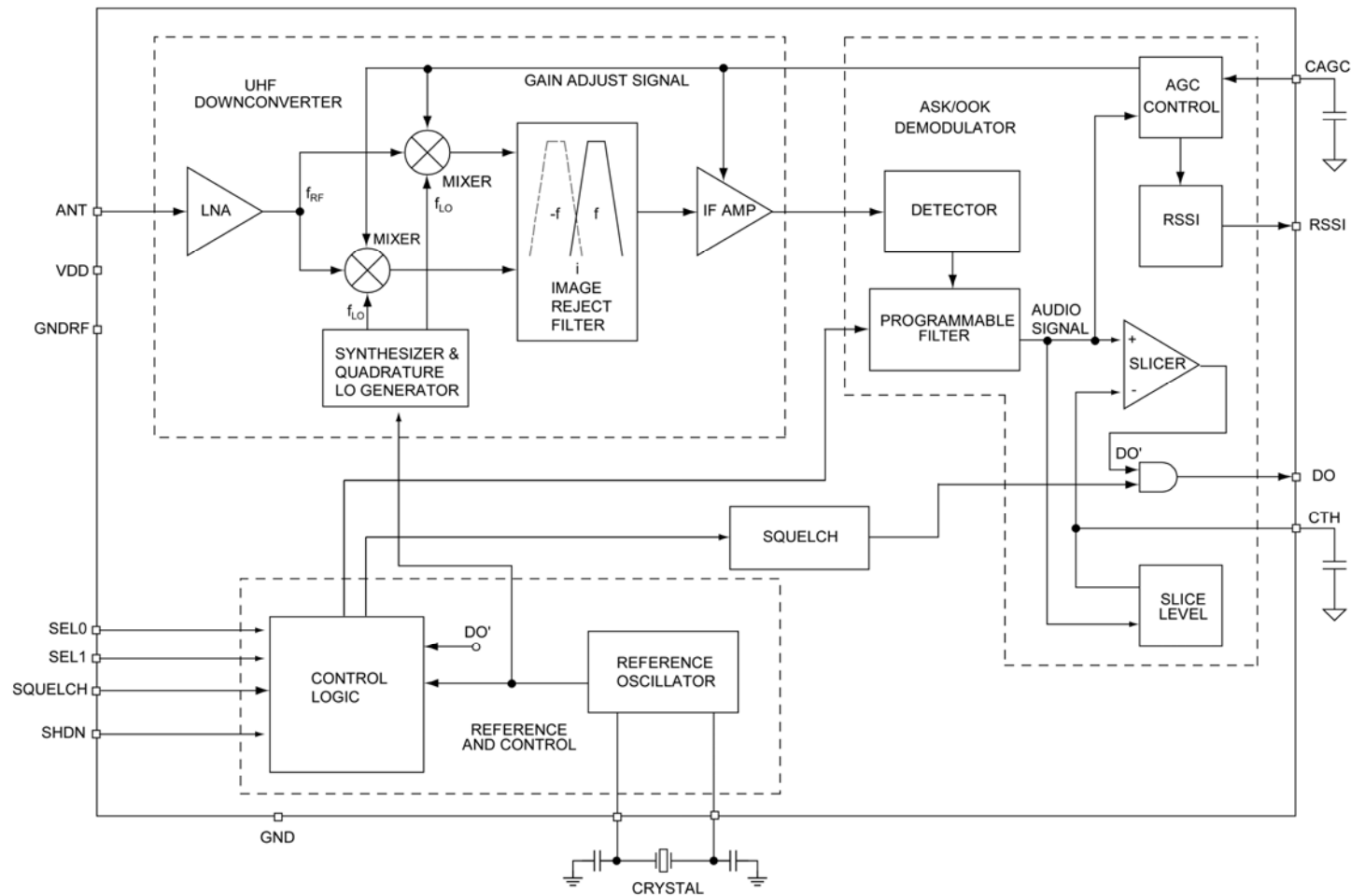
Figure 1. Simplified Block Diagram
