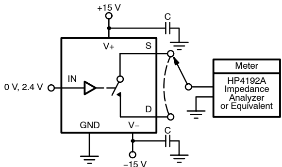
FIGURE 6. Source/Drain Capacitances
