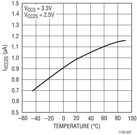
I VCC25 vs Temperature (LTC1726-2.5)
