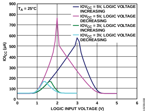
Figure 37. IOICC vs. Logic Input Voltage
