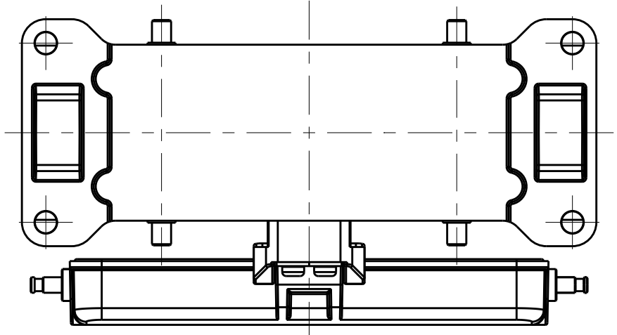
TYPE 2: HIGH BODY + METAL PROTECTITON COVER OTHER SPEC REFER TO TYPE I
