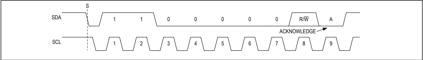
Figure 12. Slave Address Byte Example for Power Block
