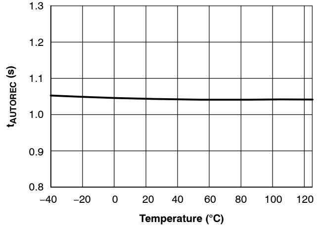
Figure 30. t AUTOREC vs. Junction Temperature
