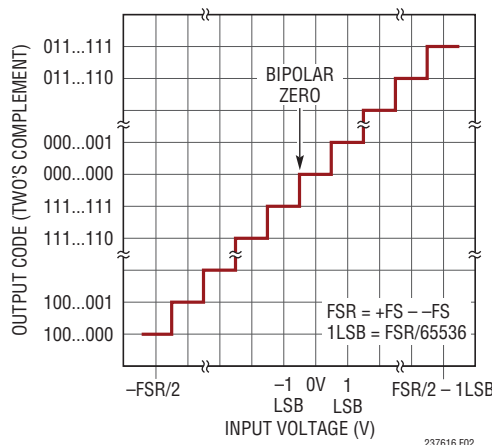
Figure 2. LTC2376-16 Transfer Function
