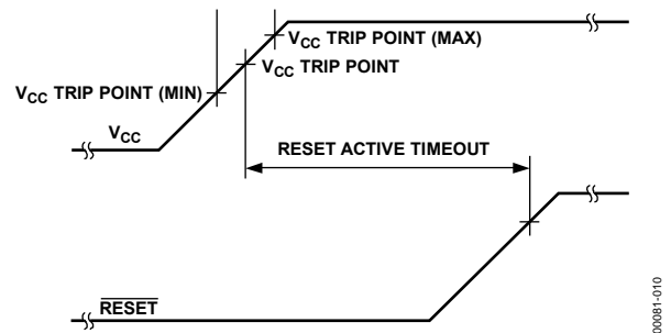
Figure 11. V_{\text{CC}} Power-Up Timing Diagram
