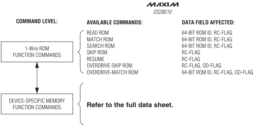
Figure 2. Hierarchical Structure for 1-Wire Protocol
