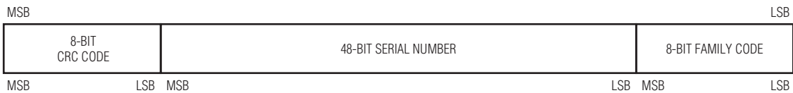
Figure 3. 64-Bit ROM ID
