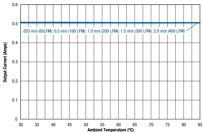
Maximum Current Temperature Derating at Sea Level (VIN = 18V, 24V, 36V, 48V, 60V, 75V airflow is from pin 1 to pin 4)
