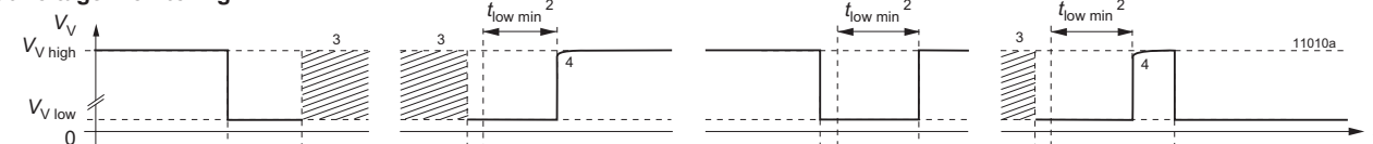
Fig. 40 Output configuration of options V0, V2 and V3
