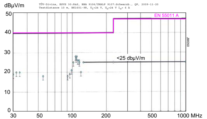
Fig. 23a Typical radiated emissions according to EN 55011/22, antenna 10 m distance, measured at V_{inom} and I_{0nom} (BK1601-9R)
