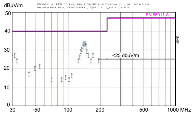
Fig. 23b Typical radiated emissions according to EN 55011/22, antenna 10 m distance, measured at V_{inom} and I_{0nom} (DK1601-9ERB1)
