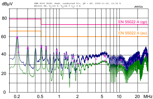
Fig. 22a Conducted emissions (peak/quasipeak and average) at the phase input according to EN 55011/22, measured at V_{inom} and I_{0nom} (BK1601-9R). The neutral line performs quite similar.
