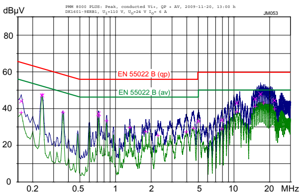
Fig. 22b Conducted emissions (peak/quasipeak and average) at the phase input according to EN 55011/22, measured at V_{inom} and I_{0nom} (DK1601-9ERB1). The neutral line performs quite similar.
