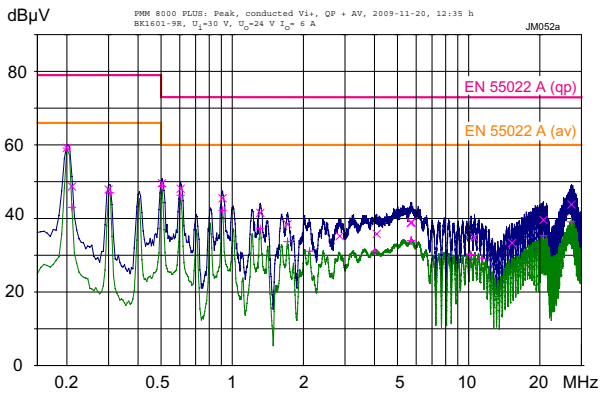
Fig. 22a Conducted emissions (peak/quasipeak and average) at the phase input according to EN 55011/22, measured at V_{inom} and I_{0nom} (BK1601-9R). The neutral line performs quite similar.
