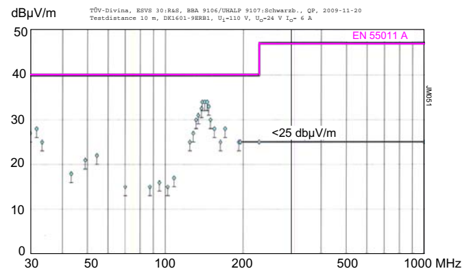
Fig. 23b Typical radiated emissions according to EN 55011/22, antenna 10 m distance, measured at V_{inm} and I_{onm} (DK1601-9ERB1)
