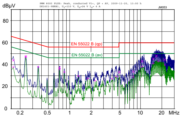
Fig. 22b Conducted emissions (peak/quasipeak and average) at the phase input according to EN 55011/22, measured at V_{inm} and I_{onm} (DK1601-9ERB1). The neutral line performs quite similar.
