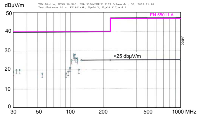
Fig. 23a Typical radiated emissions according to EN 55011/22, antenna 10 m distance, measured at V_{inm} and I_{onm} (BK1601-9R)
