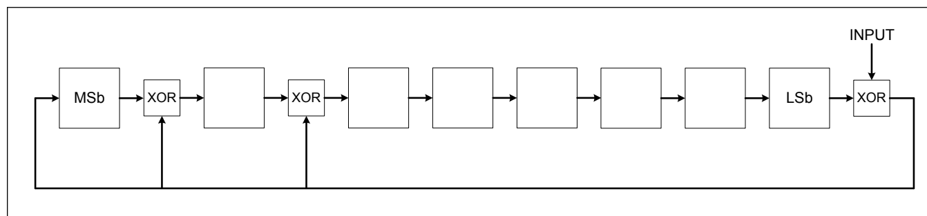
Figure 38. PEC CRC Generation Block Diagram
