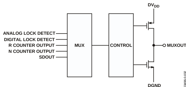
Figure 32. MUXOUT Circuit
