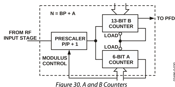
Figure 30. A and B Counters
