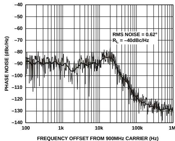
Figure 10. ADF4113 Integrated Phase Noise (900 MHz, 200 kHz, 35 kHz, Typical Lock Time: 200 \mu s)
