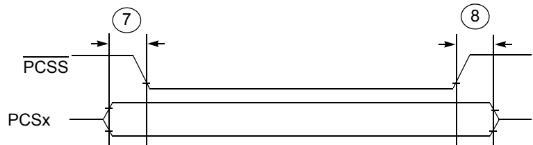
Figure 28. DSPI PCS strobe (PCSS) timing
