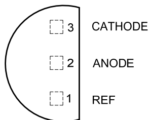
Z Package (TO-92 (Bulk Packing))
