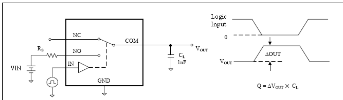
Figure 8. Charge Injection
