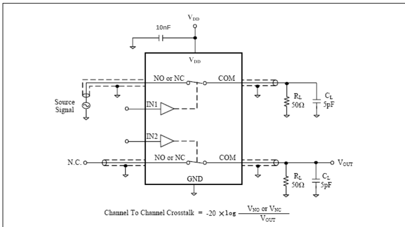
Figure 6. Channel-to-Channel Crosstalk
