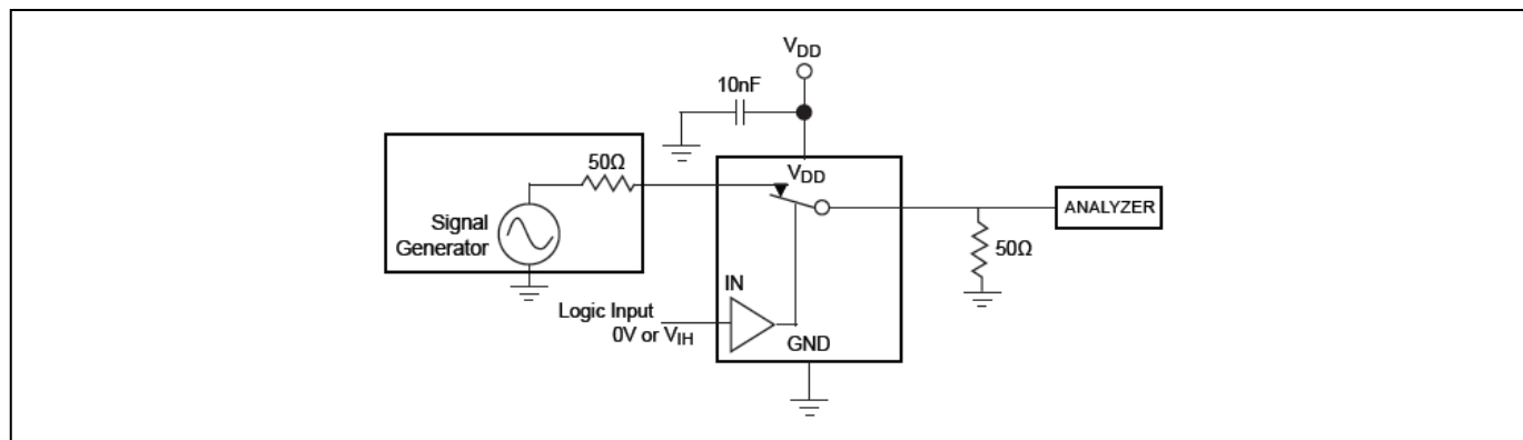
Figure 7. Bandwidth
