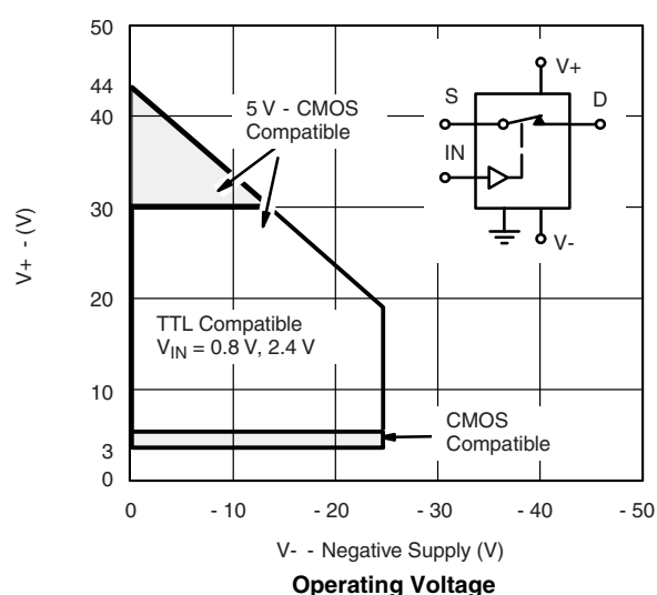
Operating Voltage
