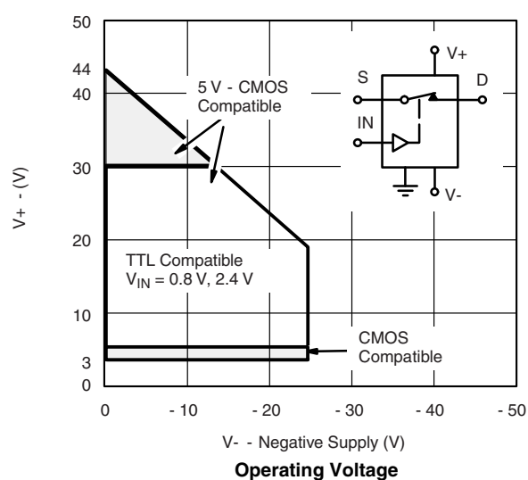
Operating Voltage
