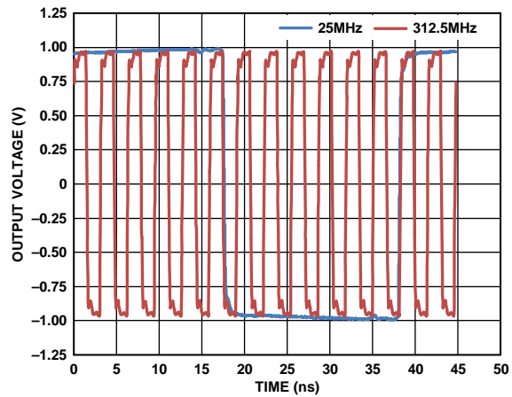
Figure 10. Output Waveform, HSTL (25 MHz, 312.5 MHz)
