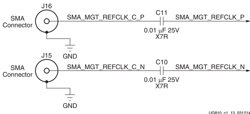
Figure 1-12: GTX SMA Clock Source
