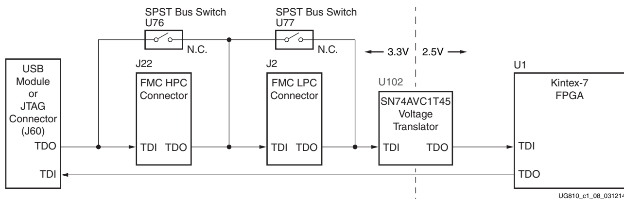
Figure 1-8: JTAG Chain Block Diagram
