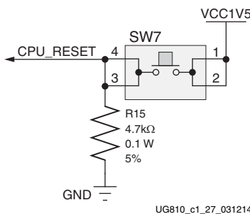
Figure 1-26: CPU Reset Pushbutton
