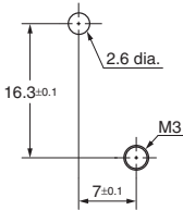
Mounting screw holes
