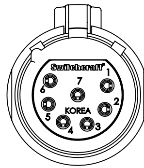
7 PIN
