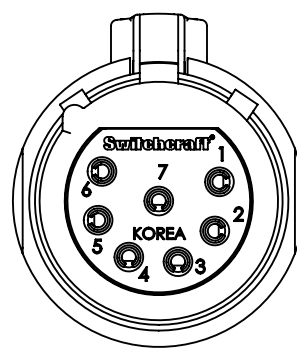
6 PIN
