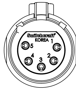
5 PIN
