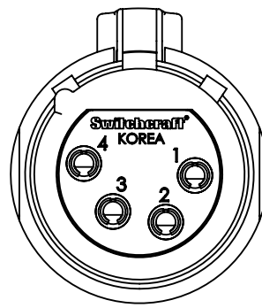
4 PIN
