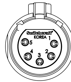
5 PIN
