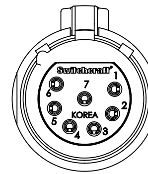
7 PIN
