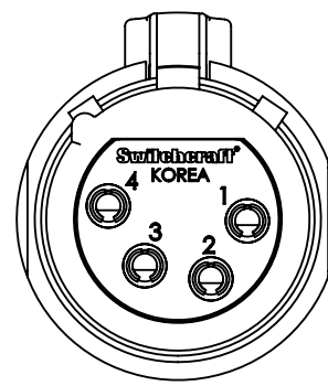
4 PIN
