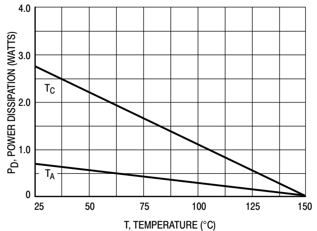
Figure 5. Power Derating
