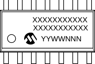
14-Lead SOIC (150 mil) (MCP3428)
