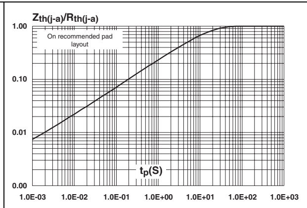
Figure 8. Relative variation of thermal impedance junction to ambient versus pulse duration (printed circuit board FR4, S_{Cu} = 1 cm 2 )
