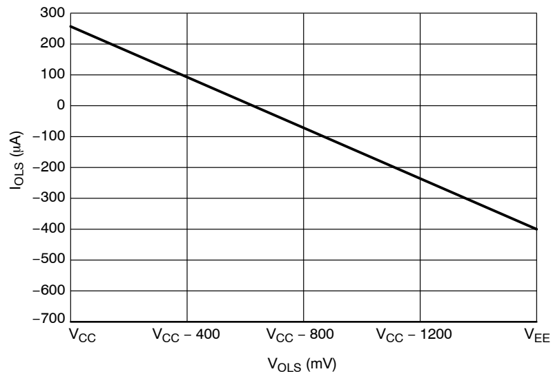
Figure 12. Typical OLS Input Current vs. OLS Input Voltage ( V_{CC} - V_{EE} = 3.3 \text{ V} @ 25^\circ C )
