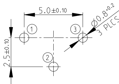
PCB MOUNTING DETAILS
