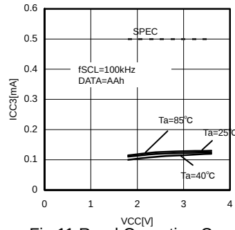
Fig.11 Read Operating Current ICC_3 ( f_{SCL}=400\text{kHz} )
