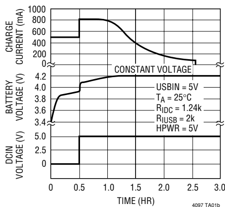
Complete Charge Cycle (1100mAh Battery)
