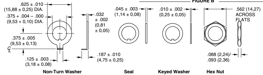
Non-Turn Washer
