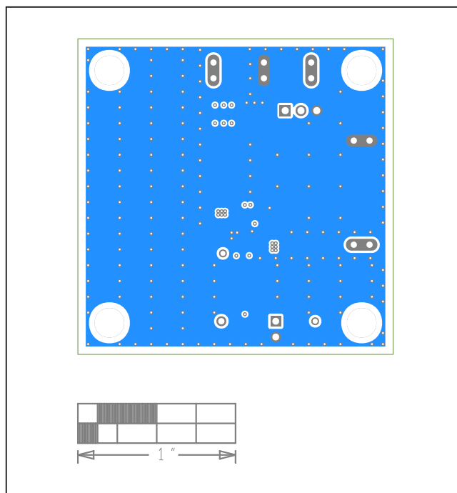
MAXM17904 EV Kit PCB Layout—Bottom Layer
