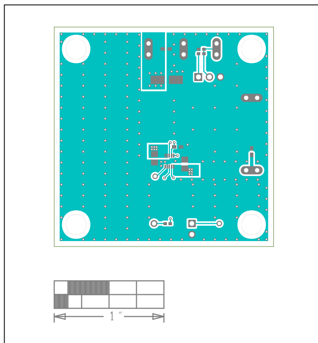
MAXM17904 EV Kit PCB Layout—Top Layer
