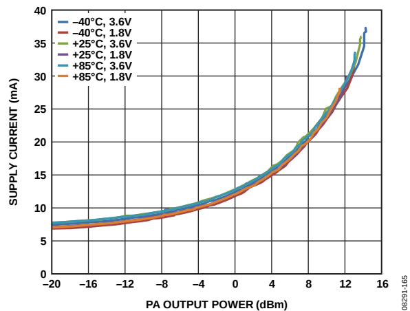
Figure 6. Single-Ended PA at 433 MHz: Supply Current vs. Output Power, Temperature, and V_{DD} (Minimum Recommended V_{DD} = 2.2 V, 1.8 V Operation Shown for Robustness)
